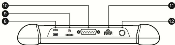
Figure 2-3 MaxiCOM MK808 Display Tablet Top View
