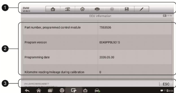
Figure 4-10 Sample ECU Information Screen
